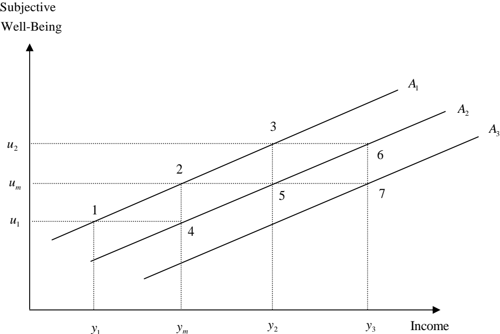
Figure 1: Subjective well-being ( u ) as a function of income ( y ) and aspiration level ( A ).
