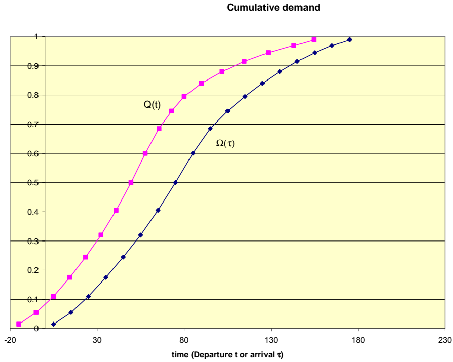
Figure 3: cumulative demand Q(t) and \Omega(\tau)
