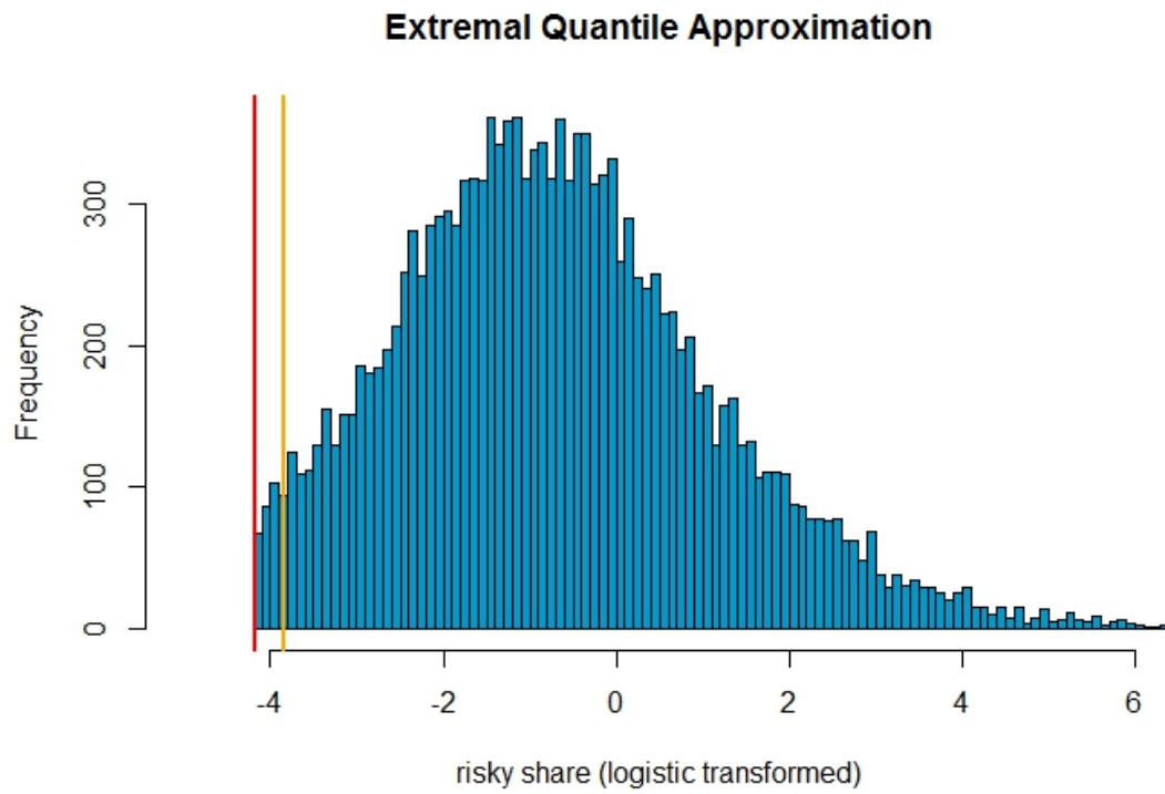
Figure 1: Intuition of Extremal Quantile Approximation
