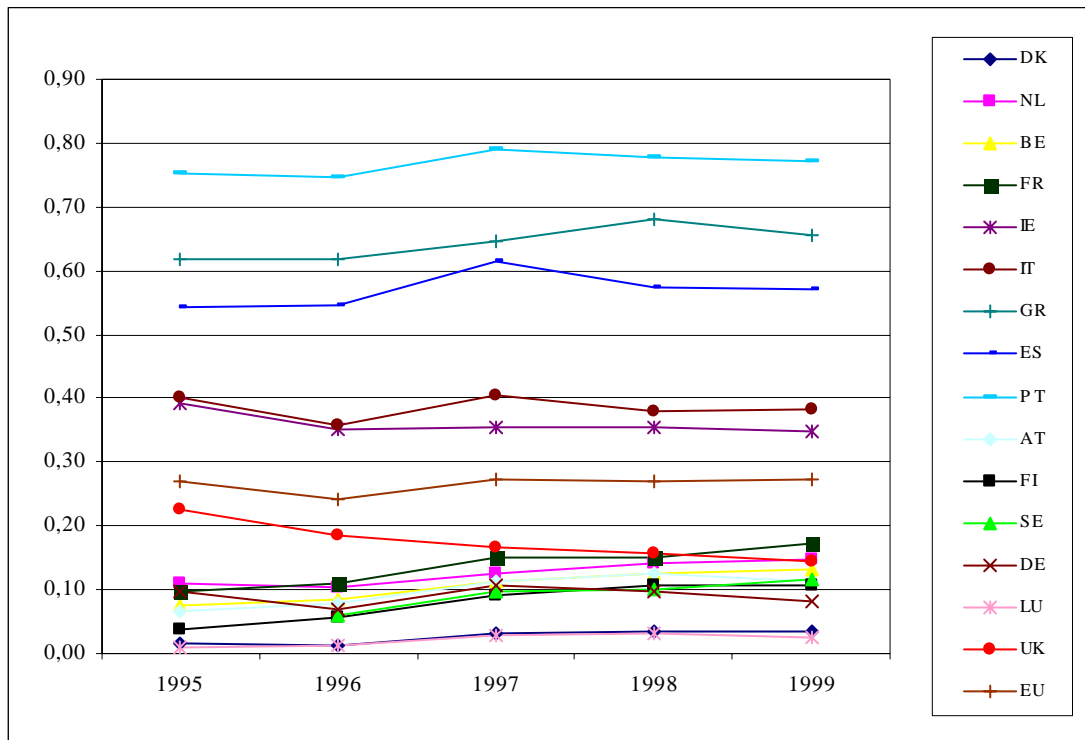
Figure 4.1.1 Poverty incidence in EU and European Countries 1995-1999. Common EU(1995) poverty line.
