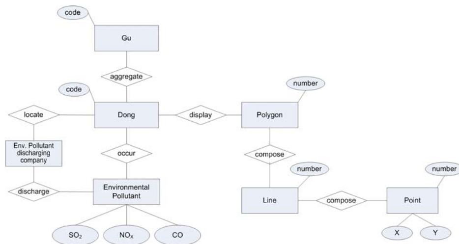
<Figure 9> Example of Entity Relationship Data Model
