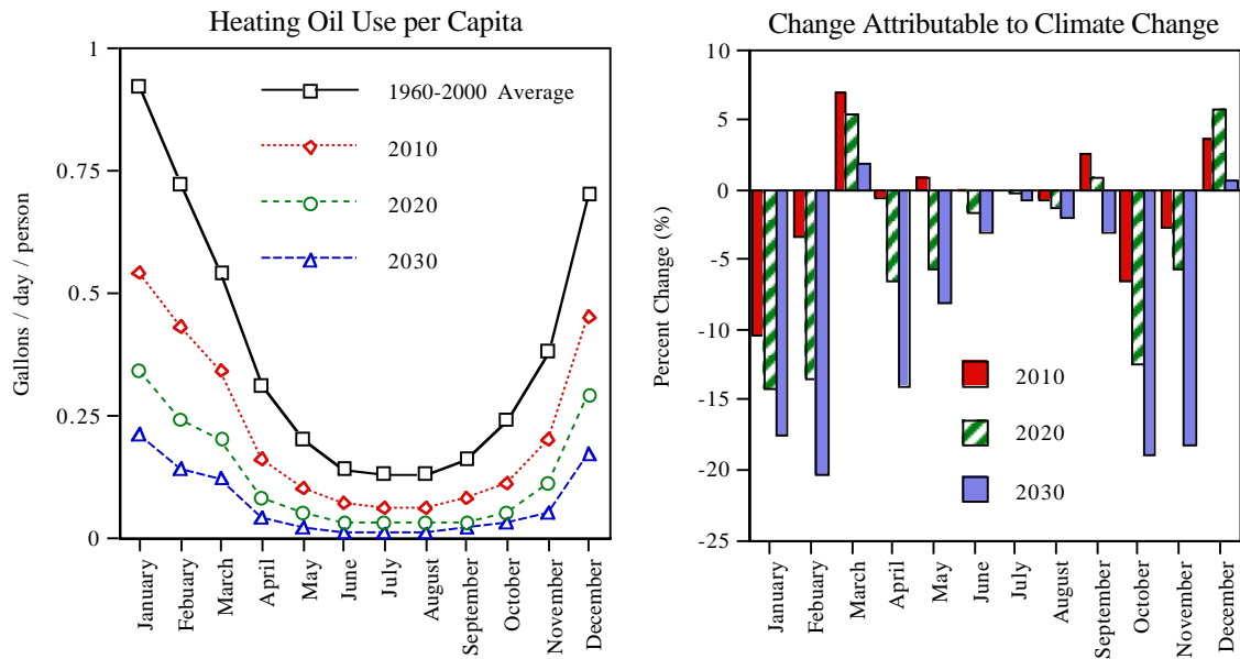
Figure 14. Residential Heating Oil Use per Capita Under Hadley Climate Scenarios (Results are Averages Across 100 Bootstrapped Climate Scenarios).
