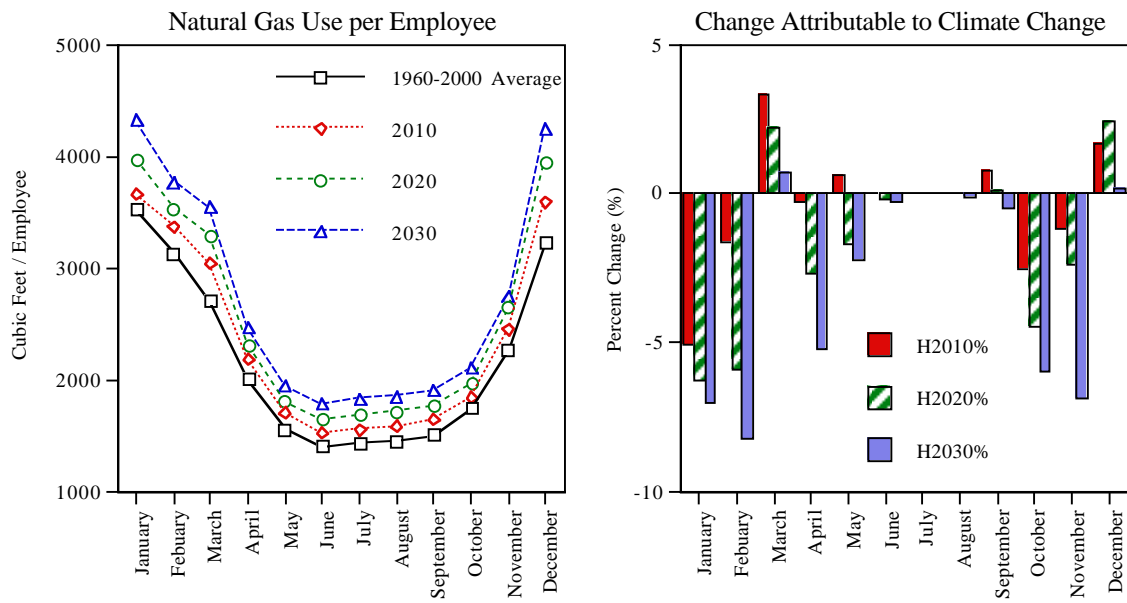
Figure 18. Commercial Natural Gas Use per Employee Under Hadley Climate Scenarios (Results are Averages Across 100 Bootstrapped Climate Scenarios).
