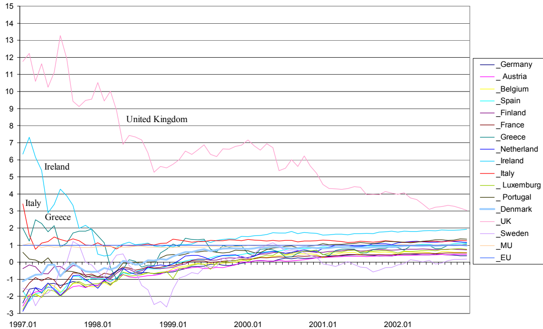
Graph 1: Evolution of B_{1996,t}^{iG} statistic
