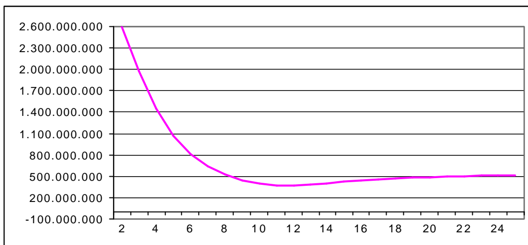
DIAGRAM 1 – Distribution of indicator I depending on parameter \beta
