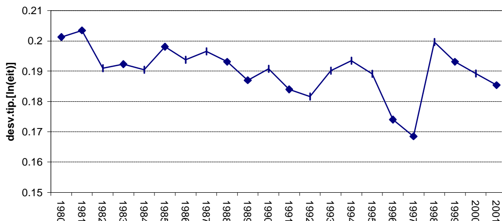
GRAPH 3: Sigma Convergence in Efficiency Levels
