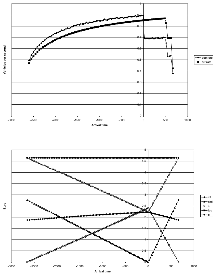
Figure 6. Arrival and departure rates by arrival time (top) and cost components by arrival time (bottom) in the approximate optimum ( N=2500 ) (plotted points are the values for drivers i=1, 25, 50, \dots, 2500 )
