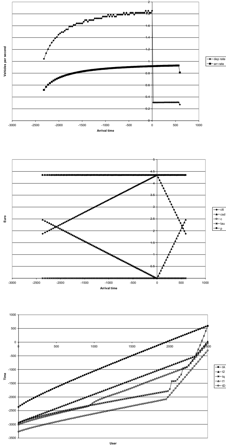
Figure 3. Arrival and departure rates by arrival time (top), cost components by arrival time (middle) and key clock-times by user (bottom) in the no-toll equilibrium ( N=2500 ) (plotted points are the values for drivers i=1,25,50,\dots,2500 )
