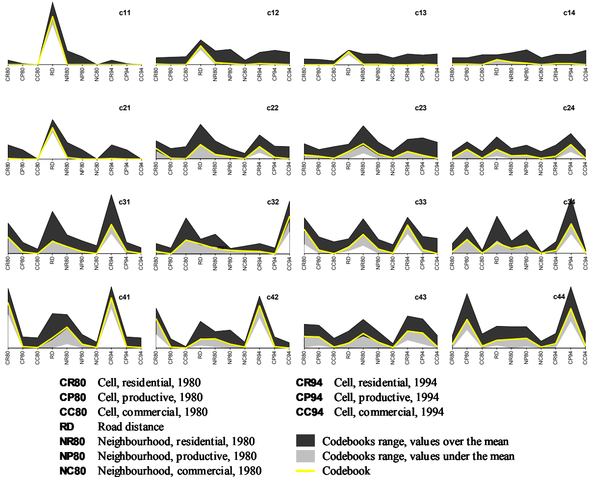
Figure 2 - The codebooks
