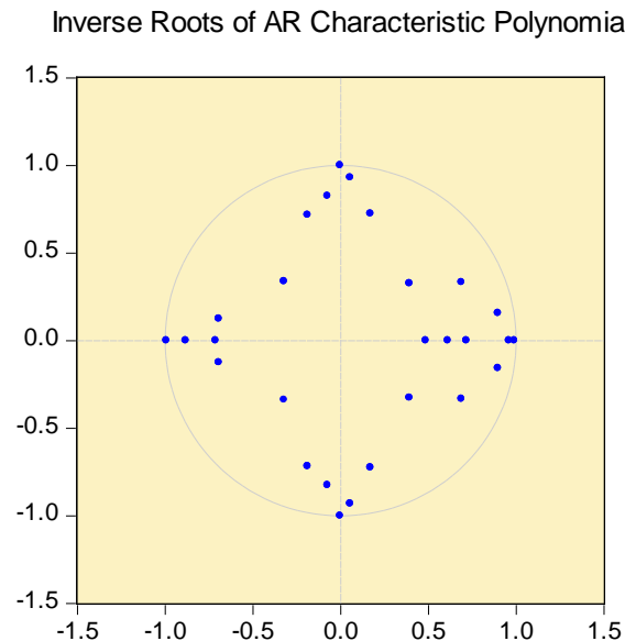
Figure 4: Stability Test of the VAR Model
