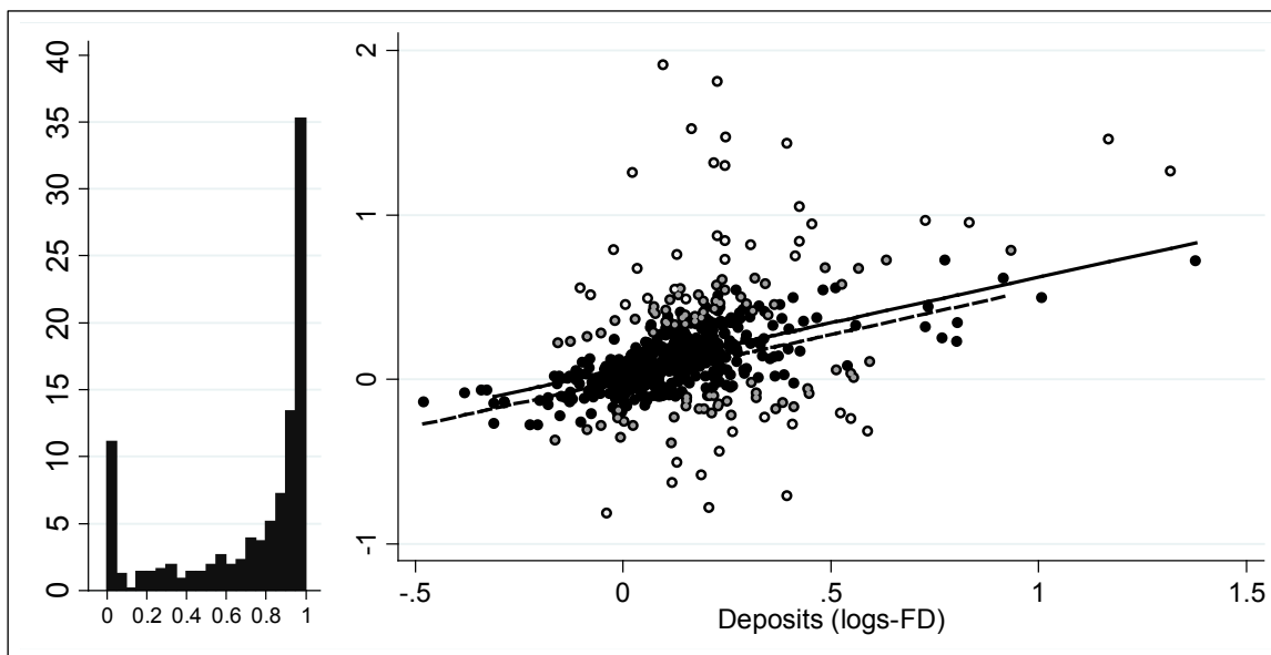
Figure 2: Outliers and LTV
