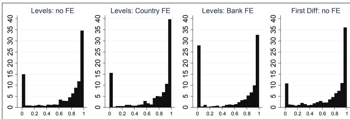
Figure 1: Distribution of Weights—Residuals
