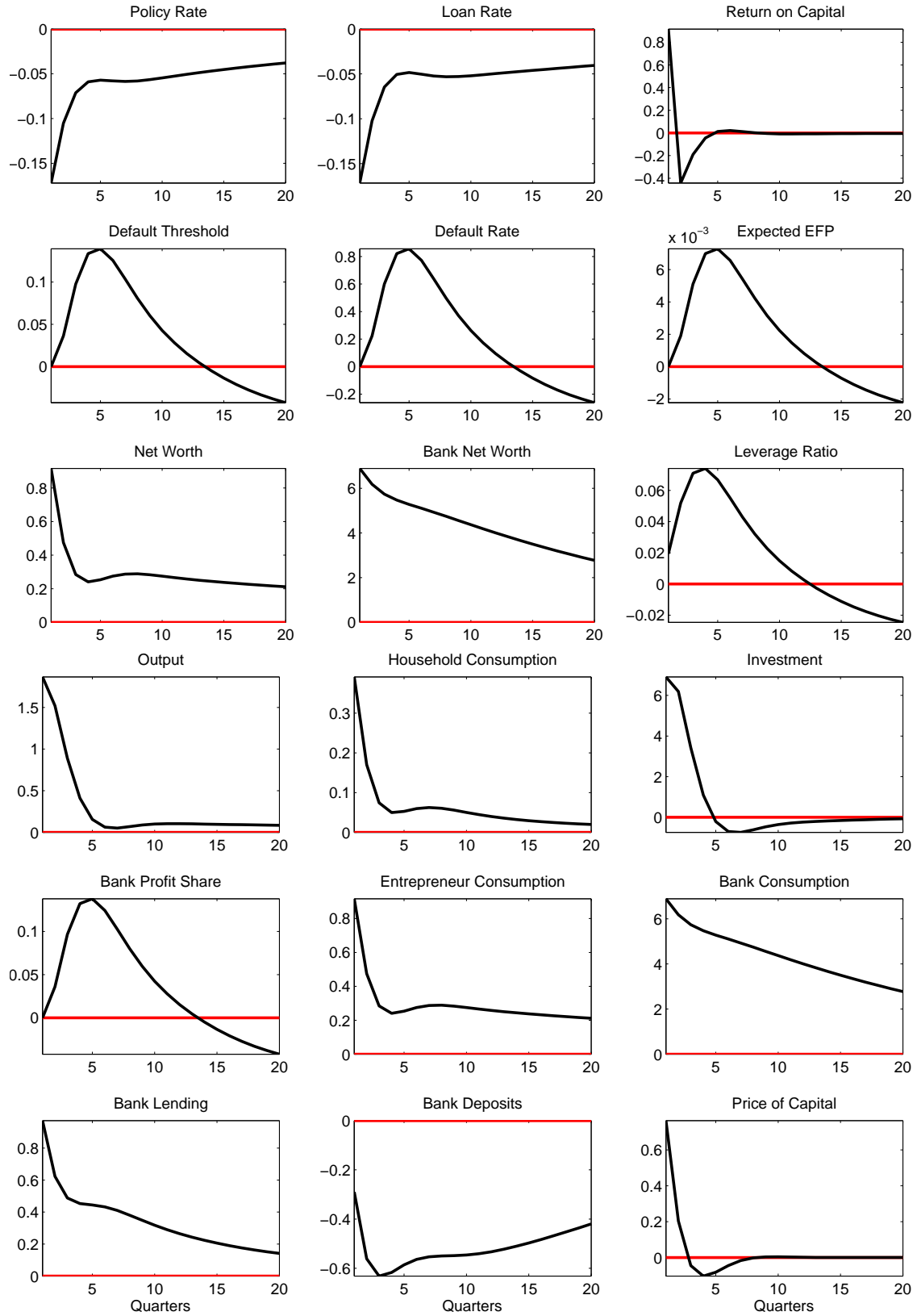
Figure 10: Selected Impulse Response Functions to an Expansionary Monetary Policy Shock of 25 Basis Points for \rho = 0.95 .
