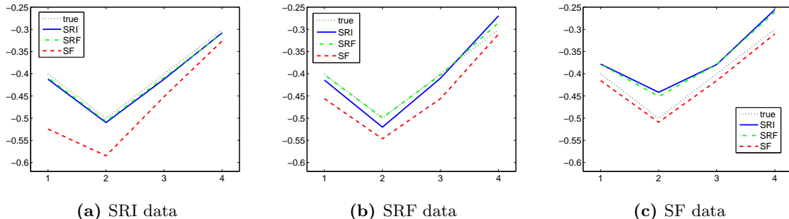
Figure 2: True and estimated average treatment effects in different models for data 1-3
