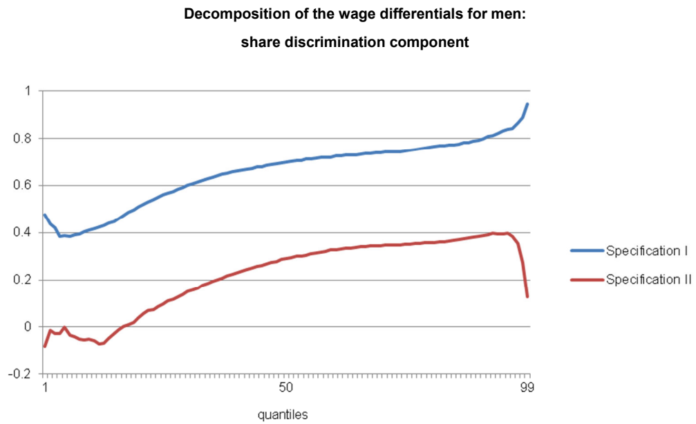
Figure 2: Discrimination component
