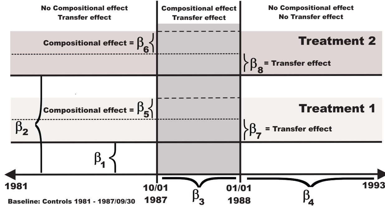
Figure 5: Research design
