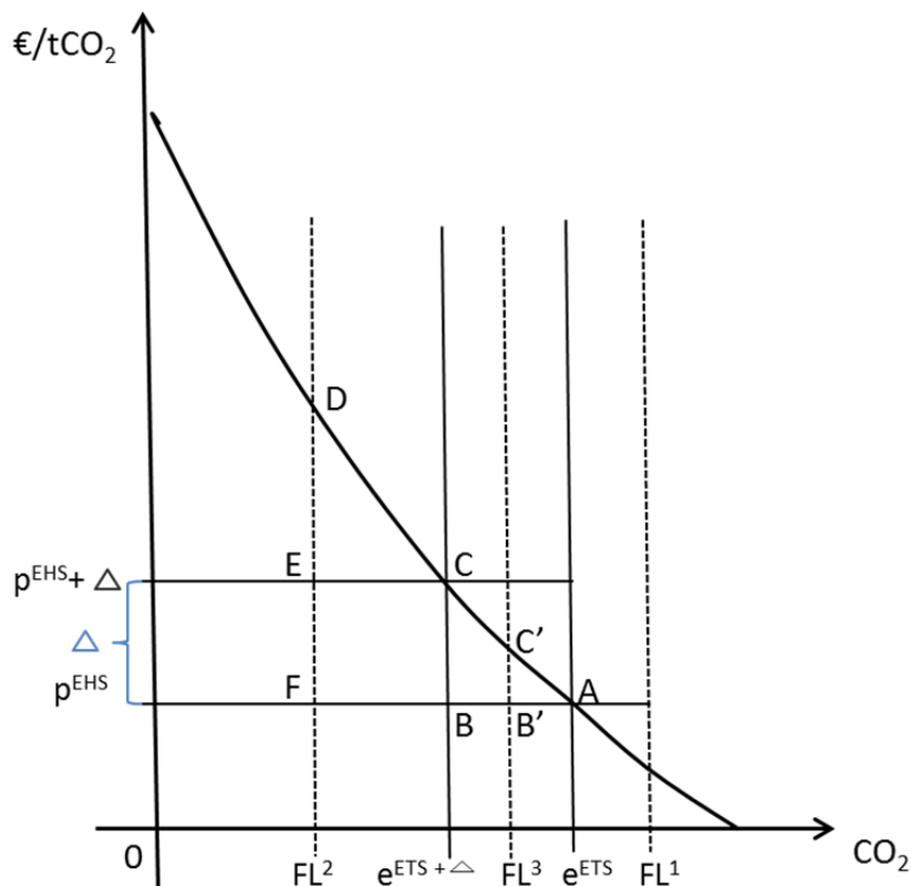
Figure 3: Marginal abatement costs of a power station
