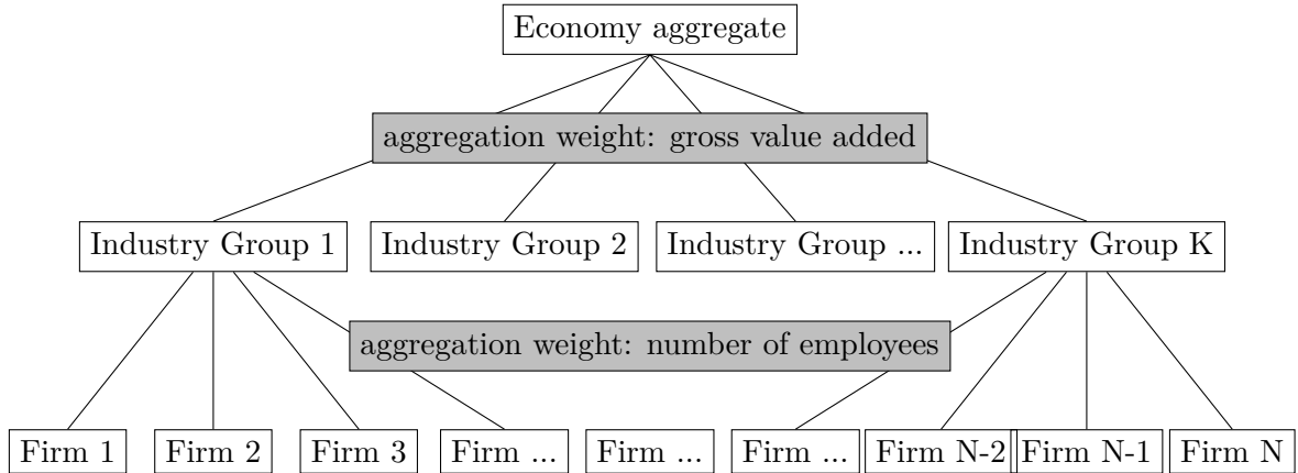
Figure 5: Aggregation scheme
