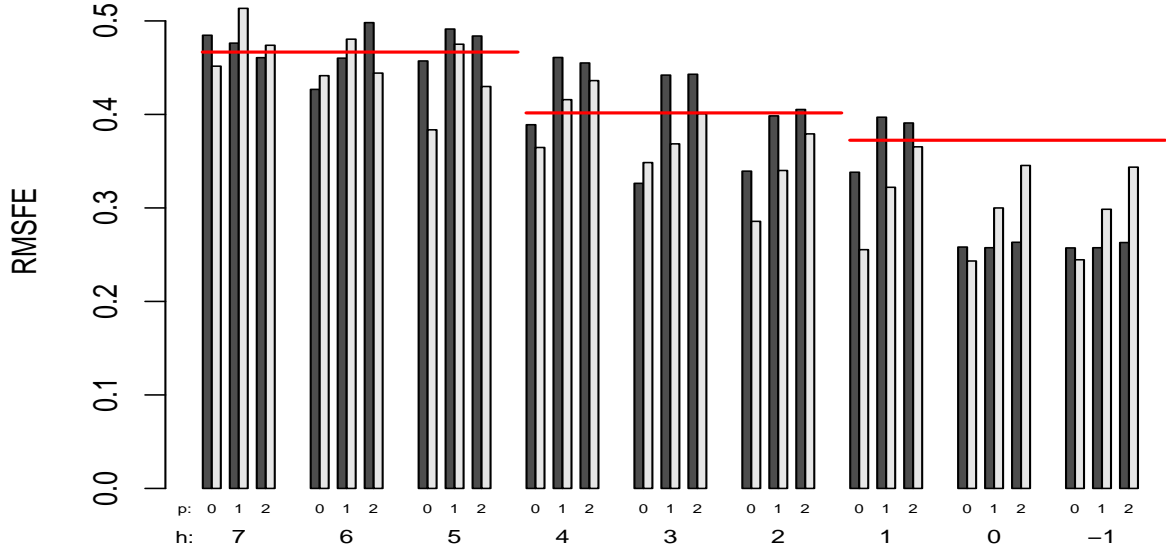
Figure 1: RMSFE: the benchmark AR(2) model (straight line); dark- and light-grey bars correspond to RMSFE of the MIDASSO and U-MIDAS-DFM models. The p parameter indicates the maximum number of lags of explanatory variables that are allowed to enter the variable selection procedure based on the elastic net. For p = 0 , as the result of skip-sampling the 559 original monthly variables are converted to 1677 quarterly variables. For p = 1 and p = 2 , the corresponding number of variables to select from is 3354 and 5031, respectively. The variable h denotes the forecast horizon that ranges from 7 months until the end of the reference quarter till -1, indicating that a forecast is made one month after the end of the reference quarter.
