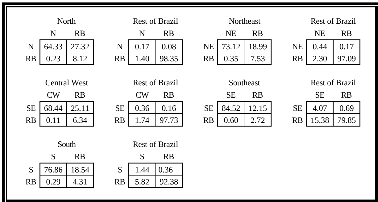
Figure 3 Schematic Representation of the Results for the 2 Regions Case
