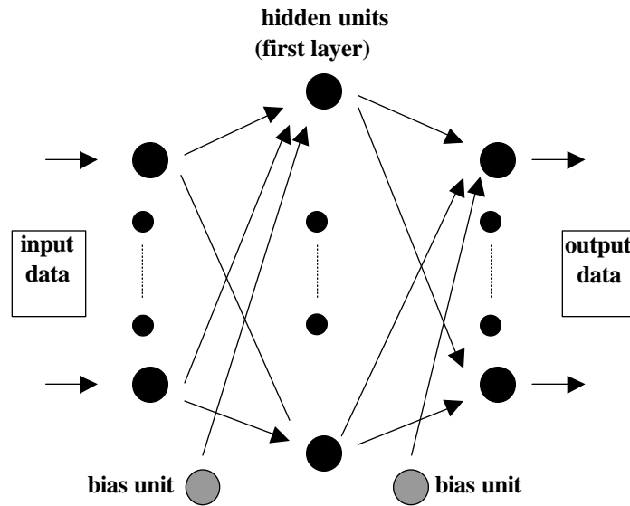
Figure 3.1. A feedforward (back-propagation) neural network architecture
