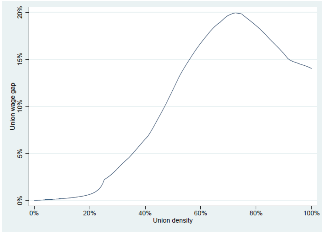
Figure 1: The Union Wage Gap Curve for Total Monthly Wages
