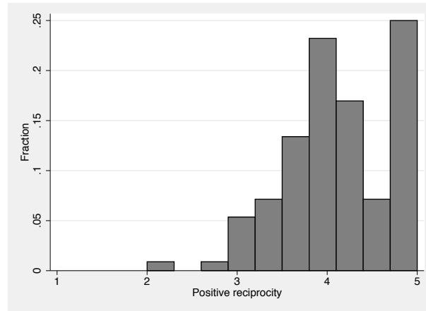
Figure 1: Distribution of reciprocity
