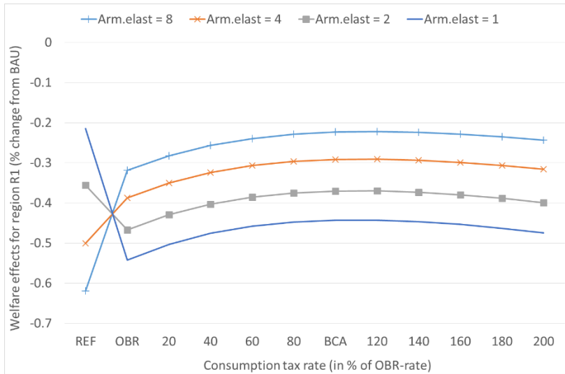
Figure 5. Welfare effects (HEV) for region R1 under different policy scenarios and Armington elasticities (% change from BAU)
