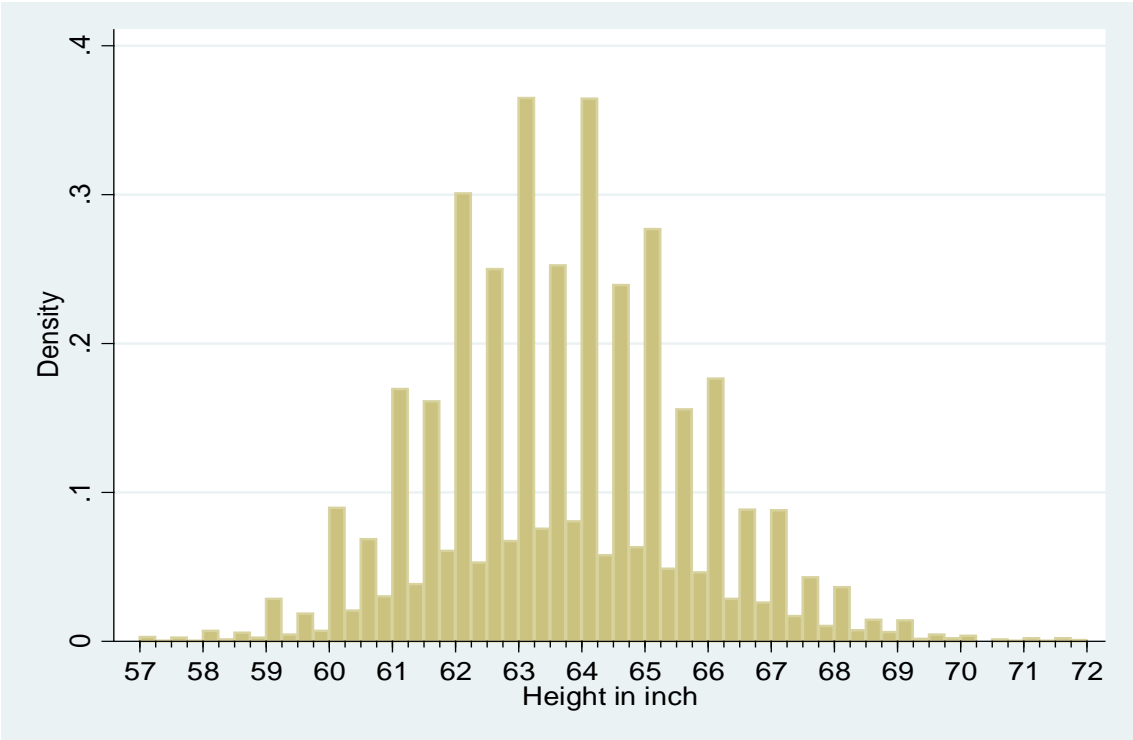
Figure 3. Height distribution in quarter inch intervals (0.635 cm)
