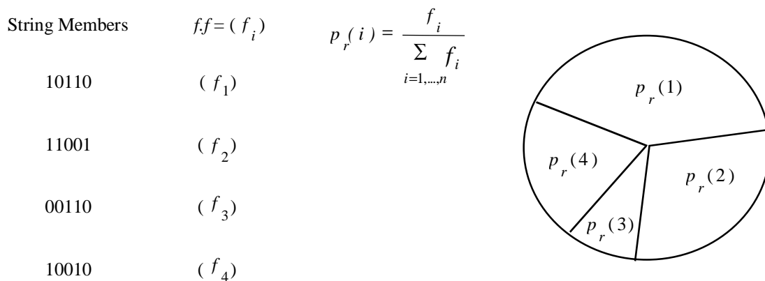
Figure 2 - Reproduction operator.
