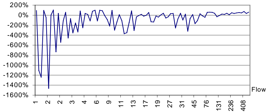
Figure 6 Relative size of residual compared to actual flow size plotted against flow. Test set with Poisson regression.
