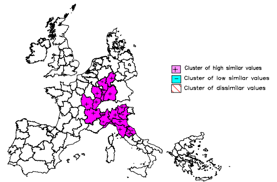
3.f.) Density function, polycentres (case 4)
