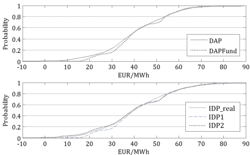
Figure 4: Cumulative Distribution Function of actual and fundamental prices
