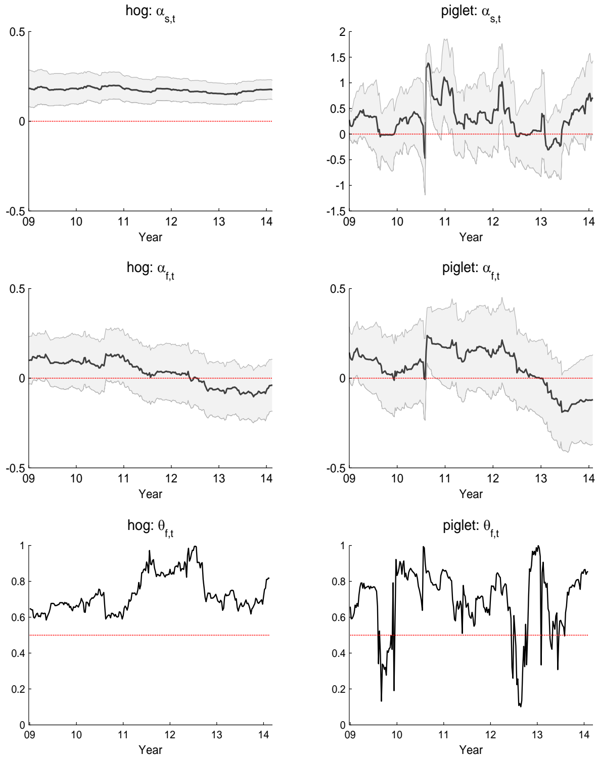
Figure 2: Time-Varying Parameters
