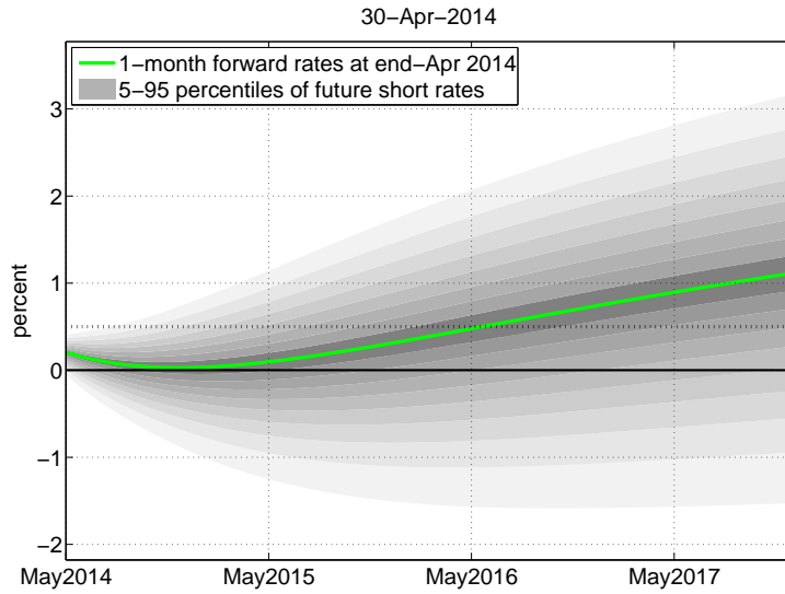
Figure 11: Conditional results of the ATSM until end 2017 based on information available at end-April 2014. Fan chart of risk-neutral conditional distributions of the short rate in gray. The green line represents the mean values of these symmetric conditional distributions.
