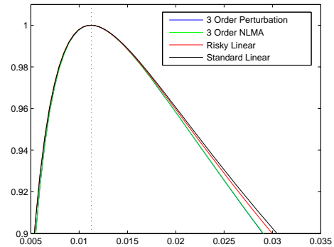
(b) Growth Shock Std. Dev. ( \bar{\sigma} )
