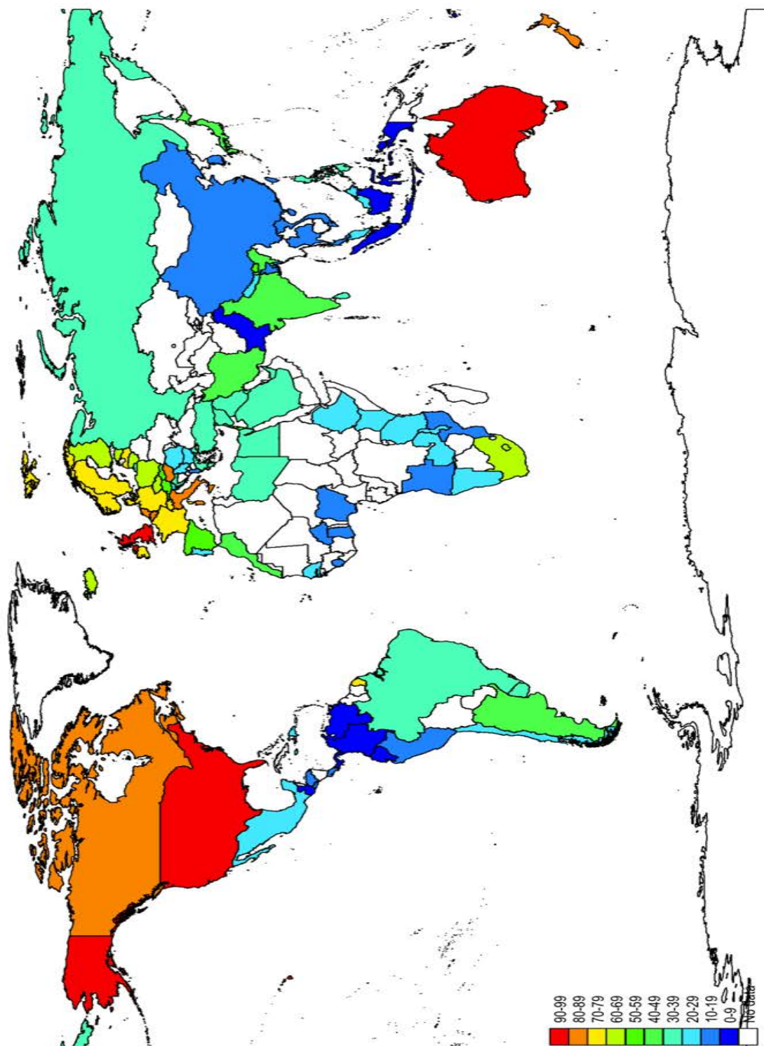
Figure 2: Individualism Scores.
