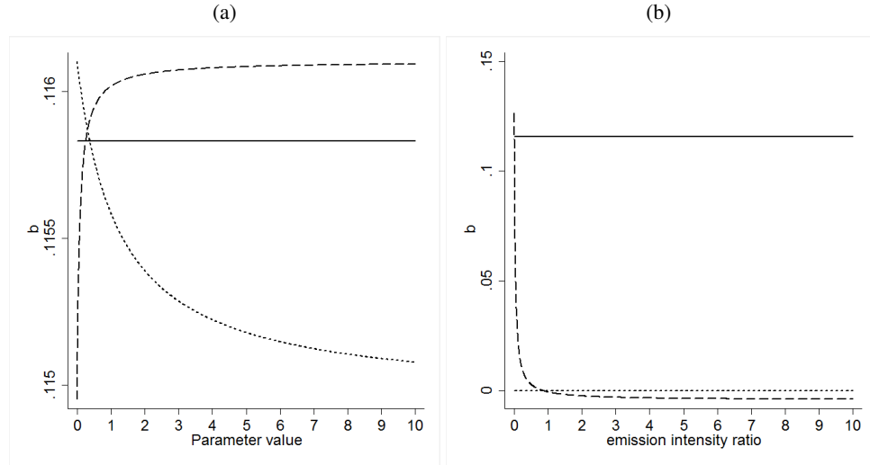
Figure 5: Numerical illustrations of the bias parameter b . Panel (a) shows the value of b with all parameters set to the reference case (solid) and as functions of the elasticity parameters \sigma_{YD} (dashed) and \zeta (dotted). Panel (b) shows the value of b as a function of the emission intensity ratio.
