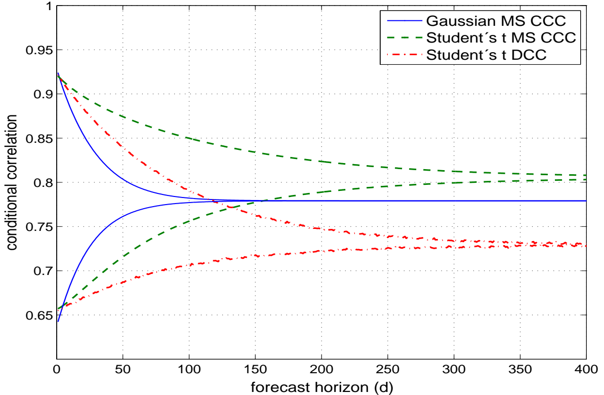
Figure 4: Shown are conditional correlations similar to the lower part of and as explained in the legend of Figure 3. The curves for the MS CCC–GARCH models reproduce those in the bottom part of Figure 3. Initial values for the conditional correlation matrix and the conditional standard deviations in the DCC model were determined such that they match those of the Student’s t MS CCC in the respective (low– and high correlation/variance) regimes.
