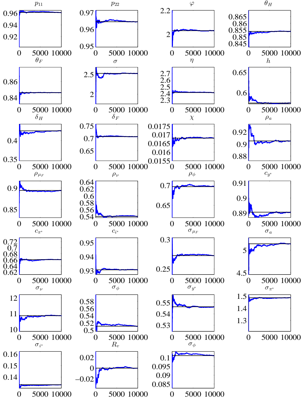
Figure 8: Recursive means of \mathcal{M}_2 . Black line indicates the posterior mean.
