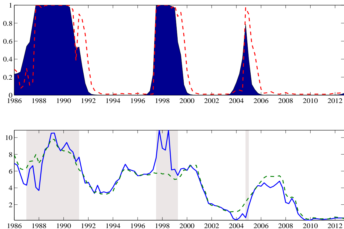
Figure 3: Top: Smoothed and not smoothed (---) probability of the “low-credibility” state P(\sigma = \sigma(2)) . Bottom: Annualized three-month interbank interest rates in per cent, HIBOR (—) and LIBOR (---). Shaded areas represent the dates in which P(\sigma_\phi(s_t) = \sigma_\phi(2)) > 0.5 .
