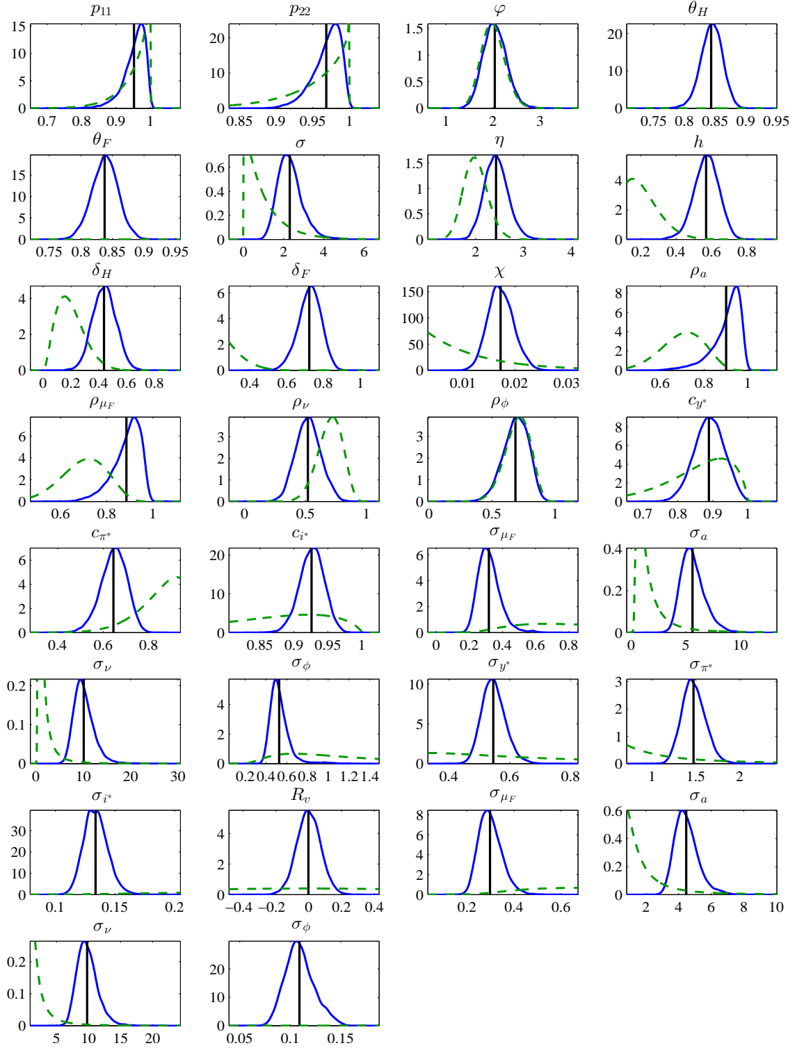
Figure 10: Prior (dashed) and posterior (solid) distributions of \mathcal{M}_3 .
