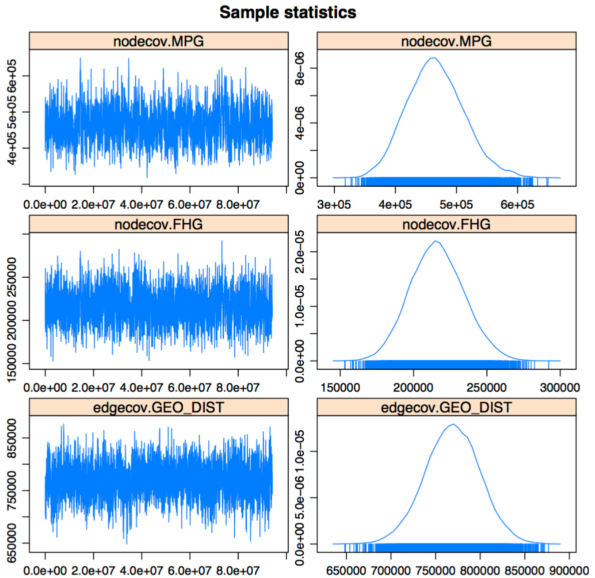
Figure 3 (b): MCMC-Statistics of exponential random graph model with dyad level, node level and structural network level variables
