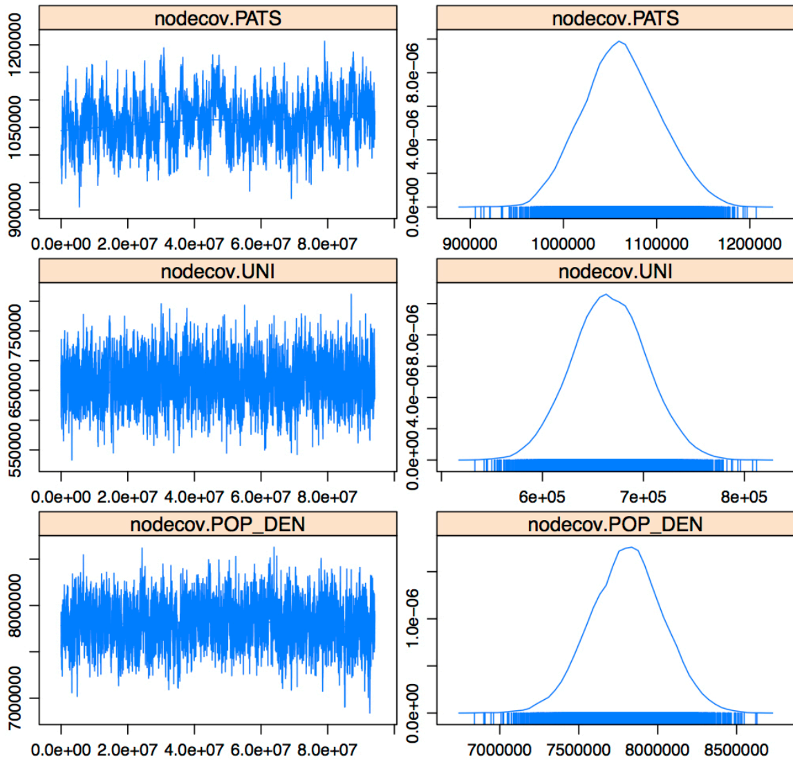
Figure 3 (a): MCMC-Statistics of exponential random graph model with dyad level, node level and structural network level variables
