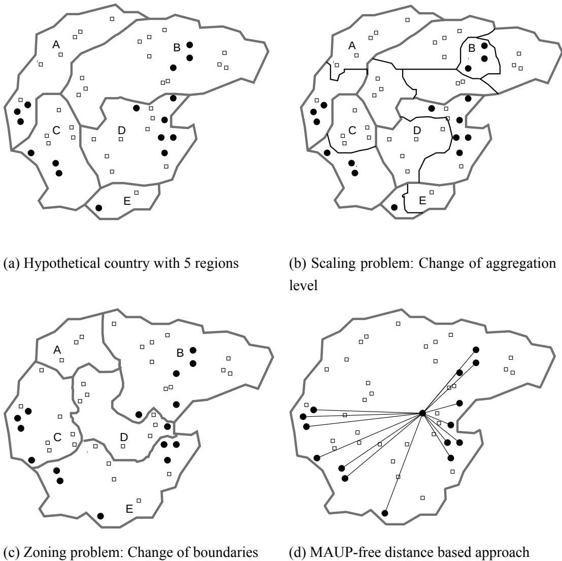
Figure 1: Measuring spatial concentration: Aggregated and none aggregated approaches
