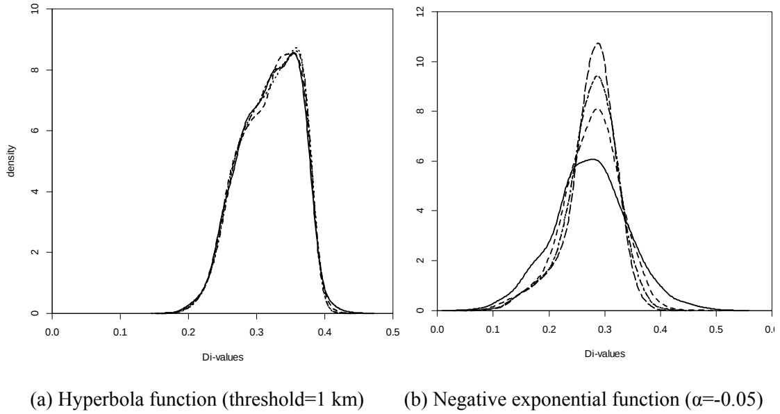
Figure 5: KDE for 2000 (solid line), 4000 (dashed line), 6000 (dotted line) and 8000 (dotted-dashed line) CSR-points.
