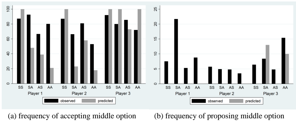
Figure 4: Accepting and Proposing middle option in part II
