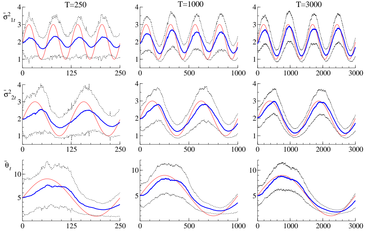
Figure 1: Simulation results under mis-specification
