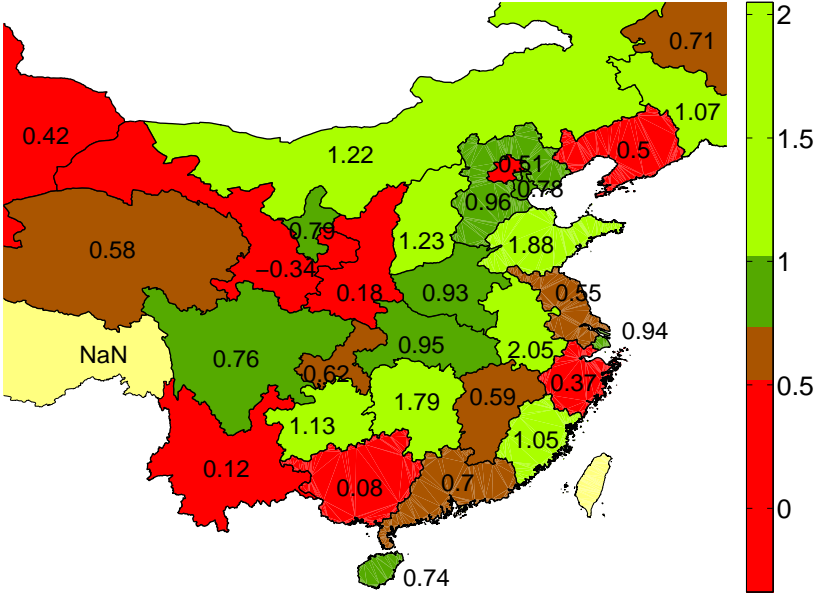
Figure 4: Net output channel \beta , 1986-2010
