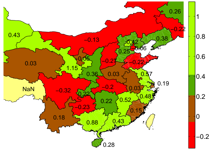
Figure 6: Interest rate channel \beta (world and domestic), 1986-2010
