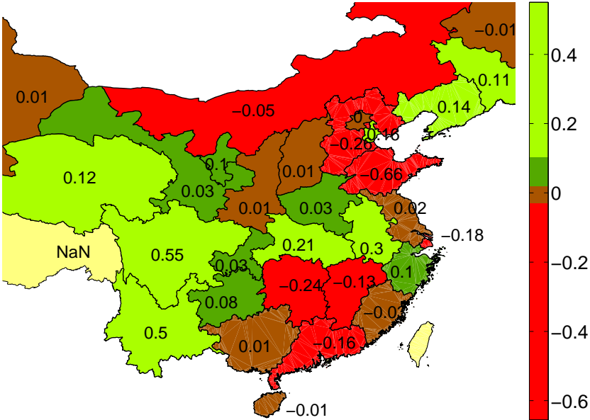
Figure 5: Internal price channel \beta , 1986-2010
