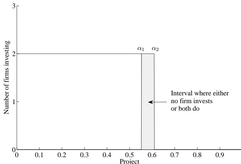
Figure 8: Violating Assumption 1.
