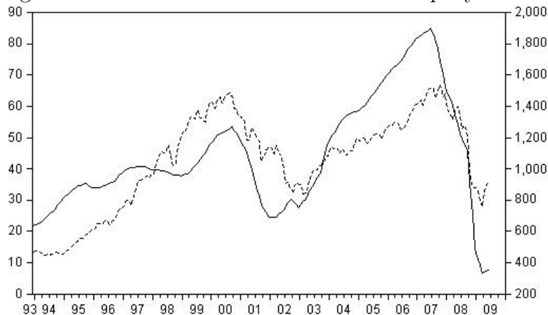
Figure 3: The S&P500 Price Index and Company Earnings
