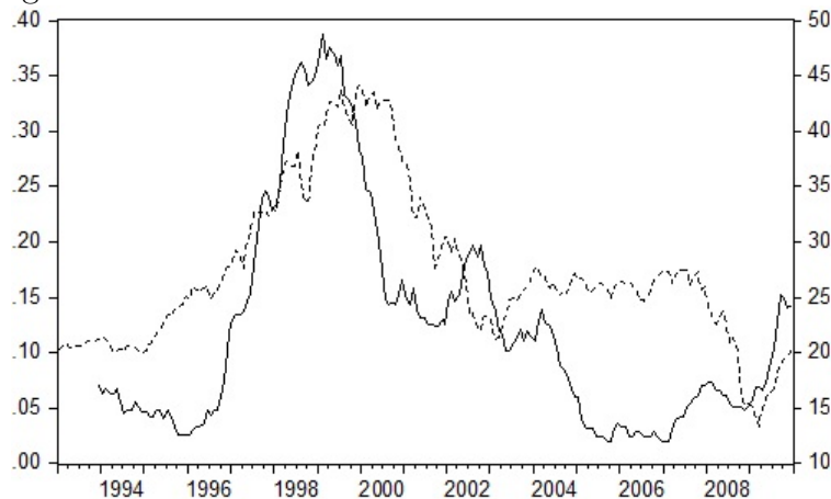
Figure 4: The S&P500 PE Ratio and Benchmark Valuation
