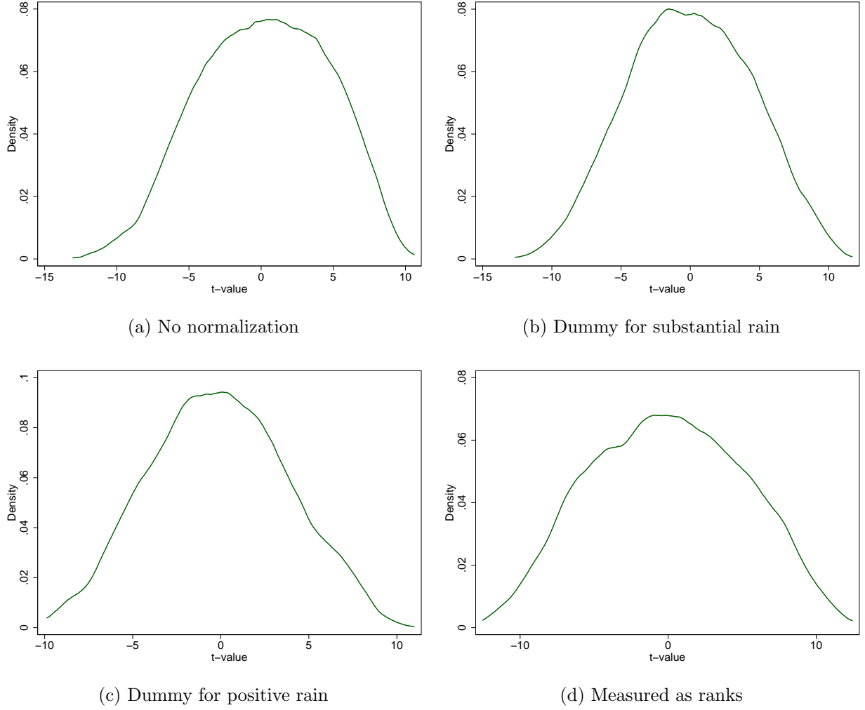
Figure 4: Distribution of the t-values
