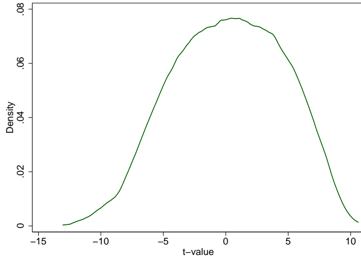
Figure 1: Regression coefficients
