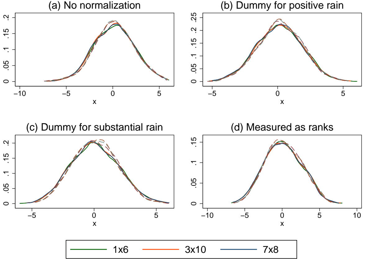
Figure 8: Distribution of t-values controlling for spatio-temporal trends
