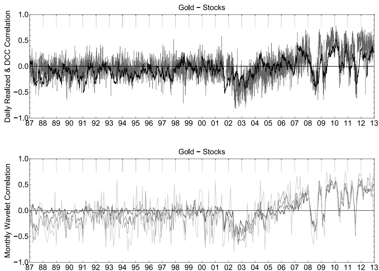
Figure 3: Dynamics in gold – stocks correlations. The upper panel contains the realized correlation for each day of the sample (grey line) and daily correlations estimated from the DCC GARCH model (black line). The lower panel contains time-frequency correlations based on the wavelet correlation estimates from high-frequency data for each month separately. We report correlation dynamics at 10-minute, 40-minute, 2.66 hour (approximate), and 1.6-day (approximate) horizons depicted by the thick black to thin black lines.
