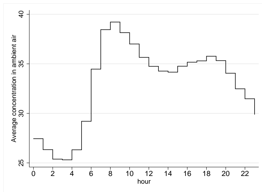
(a) PM10
