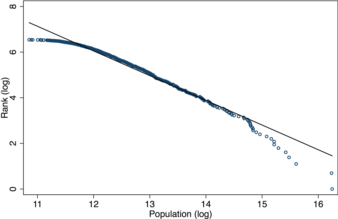
Fig. 2. Population distribution across 692 functional urban areas in Europe, 2006. Horizontal axis depicts the natural logarithm of the city population. Vertical axis depicts the natural logarithm of the city’s rank when all cities are ordered according to their population size (see Table 1). The solid line is the OLS regression line (assuming a common intercept).
