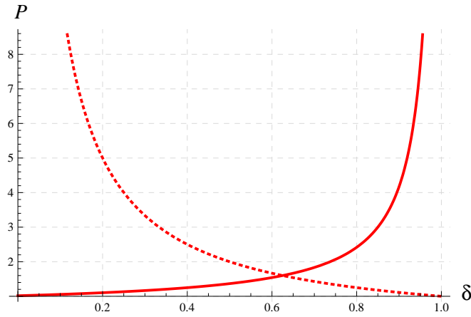
Figure 6: Equilibrium attitude towards the environment; parameters \varepsilon = 0.05, \rho = 0.05, A = 1.5, \gamma = 2, \xi_P = -1 ; solid line P(\delta) from (27), dashed line \delta(P) as assumed
