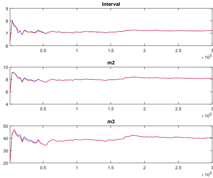
Figure 11: Convergence diagnostics - Spain
