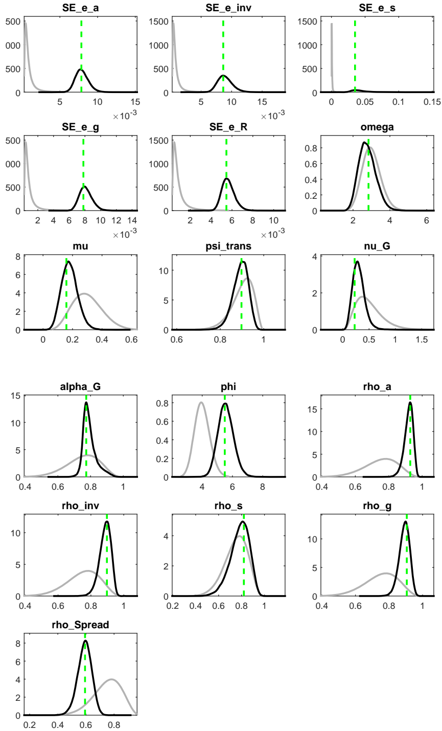
Figure 8: Priors and Posteriors - Portugal
